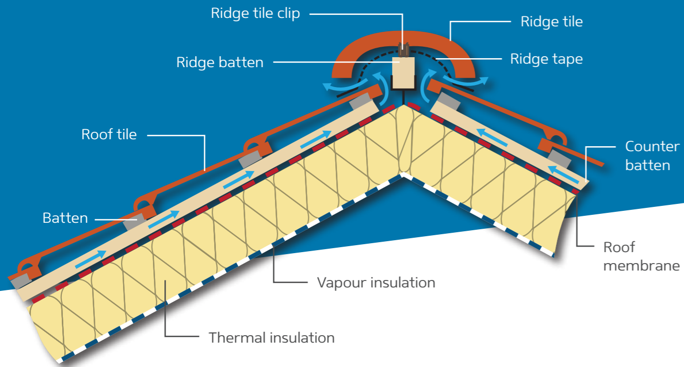
Instruction of the Eurovent® ridge tape installation
