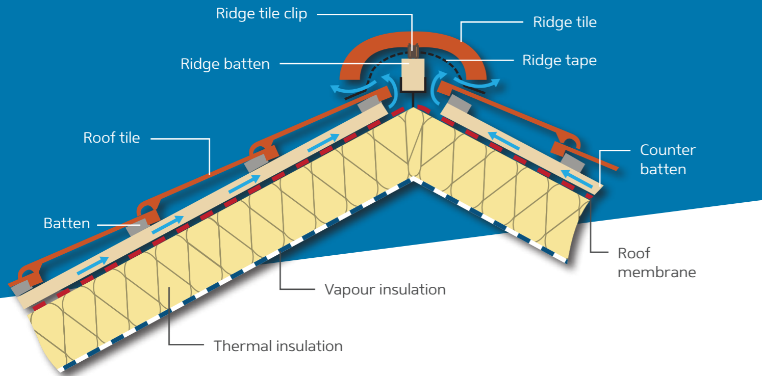
Instruction of the Eurovent® ridge tape installation
